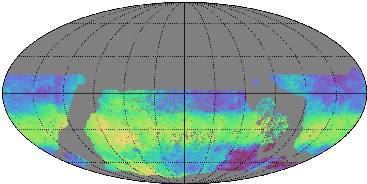
too_elab_r256_d3_ugrizy_v3.4_10yrs WFD u band: Median HA
