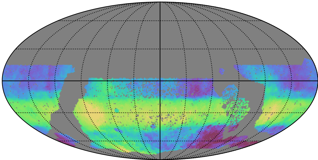
too_elab_r256_d3_ugrizy_v3.4_10yrs WFD r band: Median HA
