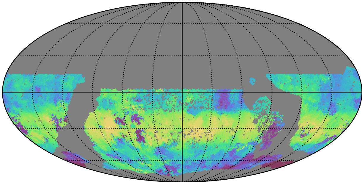
too_elab_r256_d3_ugrizy_v3.4_10yrs WFD g band: Median HA
