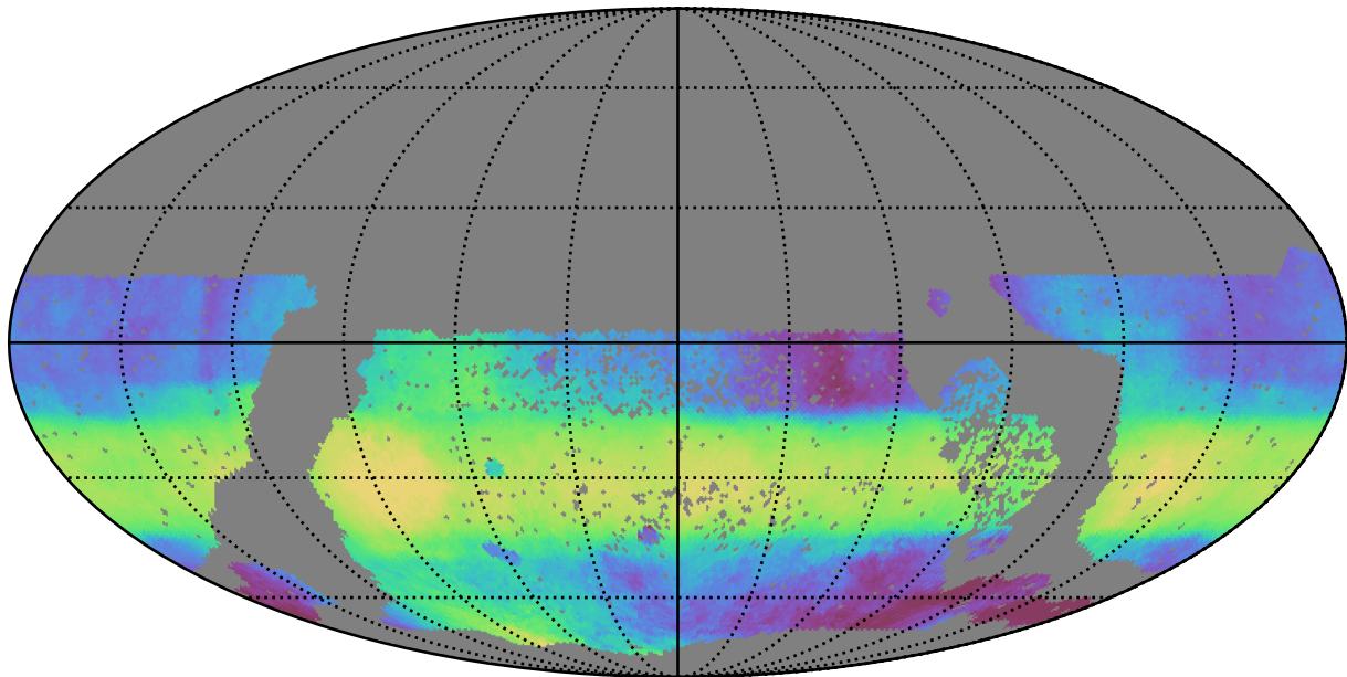
too_elab_r256_d3_ugrizy_v3.4_10yrs WFD all bands: Median HA
