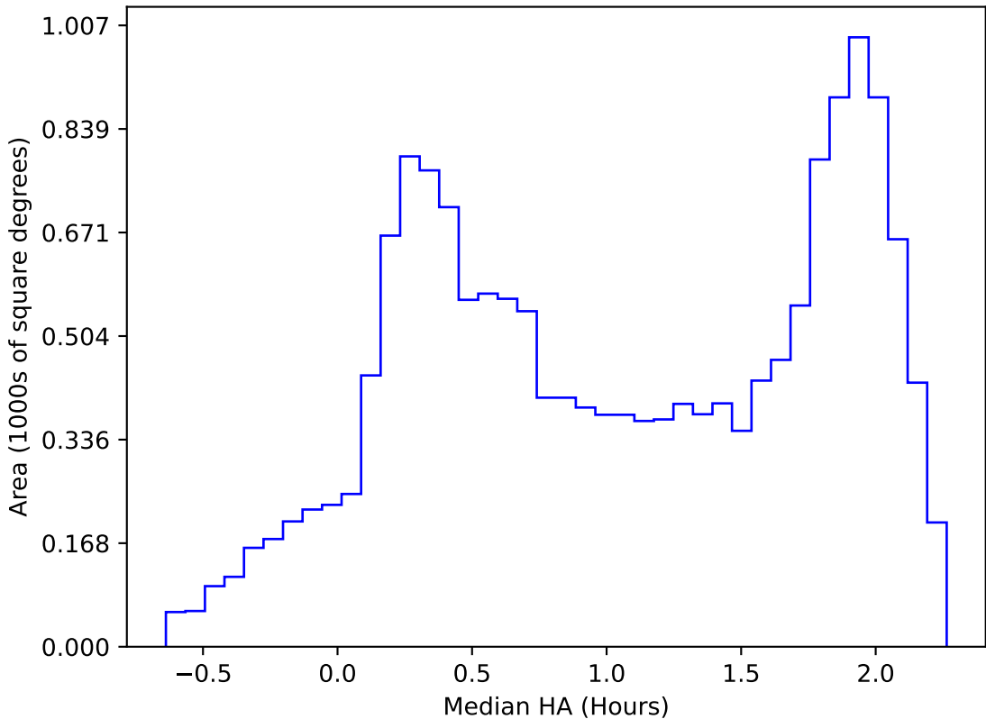
too_elab_r256_d3_ugrizy_v3.4_10yrs WFD all bands: Median HA
