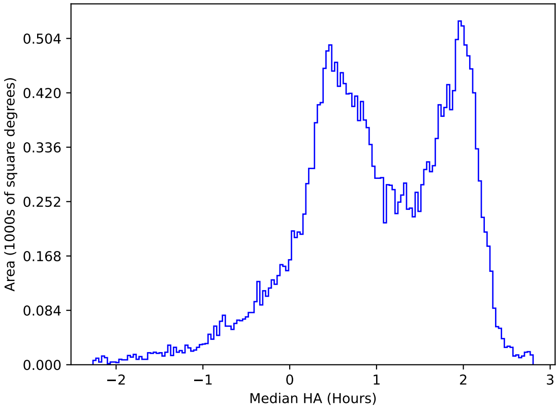
too_elab_r256_d3_ugrizy_v3.4_10yrs All sky z band: Median HA
