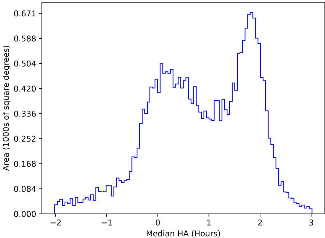
too_elab_r256_d3_ugrizy_v3.4_10yrs All sky u band: Median HA
