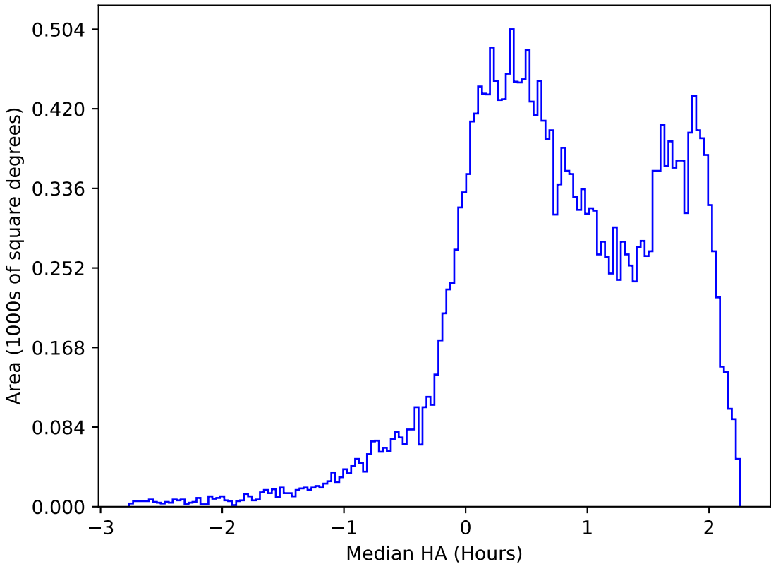
too_elab_r256_d3_ugrizy_v3.4_10yrs All sky r band: Median HA
