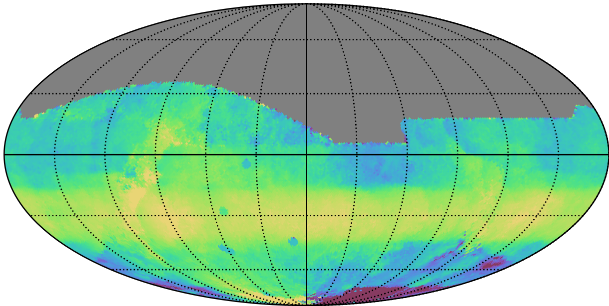
too_elab_r256_d3_ugrizy_v3.4_10yrs All sky i band: Median HA
