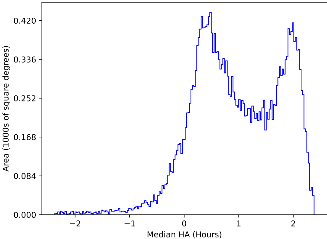
too_elab_r256_d3_ugrizy_v3.4_10yrs All sky i band: Median HA
