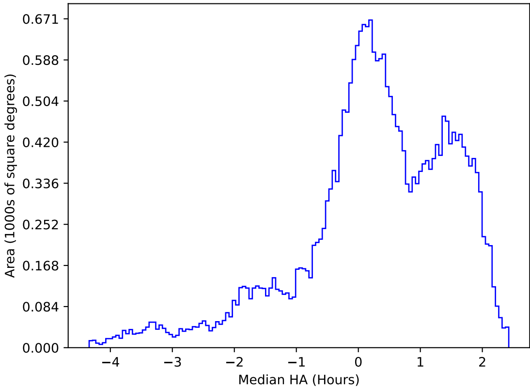
too_elab_r256_d3_ugrizy_v3.4_10yrs All sky g band: Median HA
