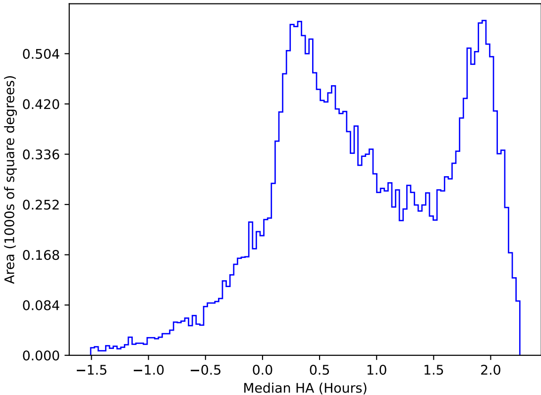
too_elab_r256_d3_ugrizy_v3.4_10yrs All sky all bands: Median HA
