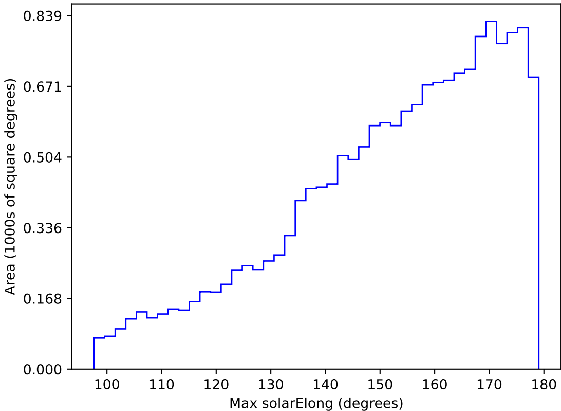
too_elab_r256_d3_ugrizy_v3.4_10yrs WFD u band: Max solarElong
