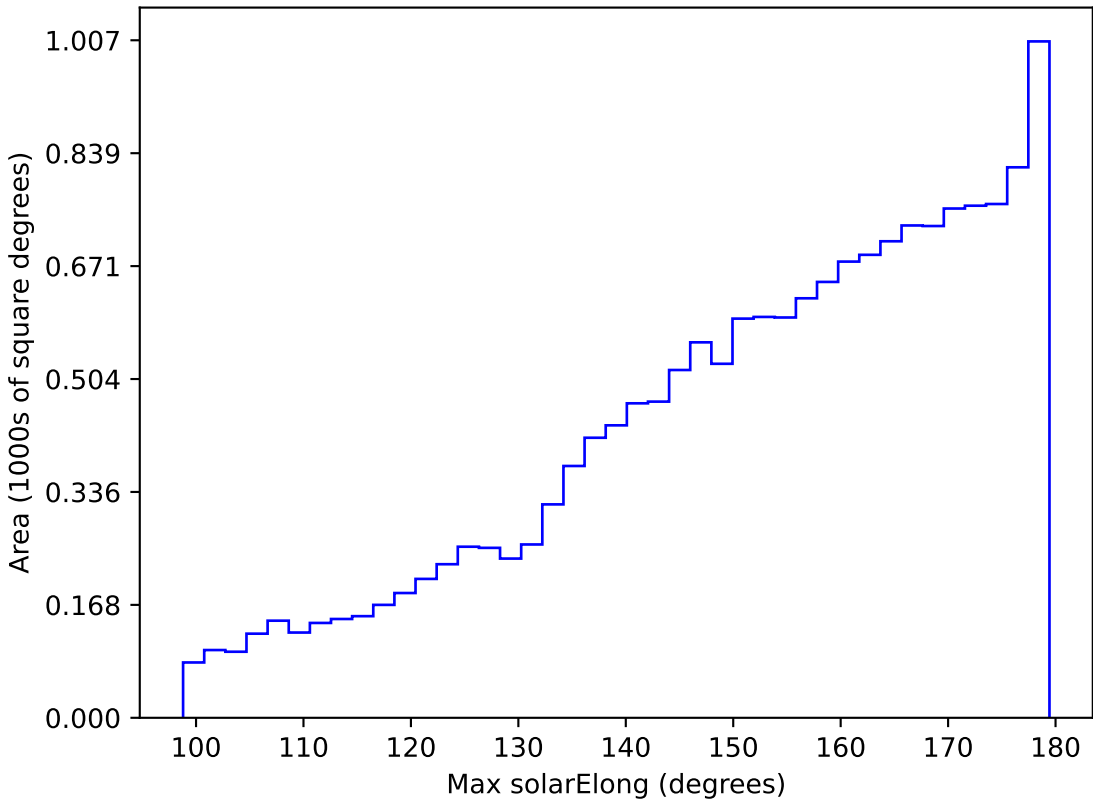
too_elab_r256_d3_ugrizy_v3.4_10yrs WFD i band: Max solarElong
