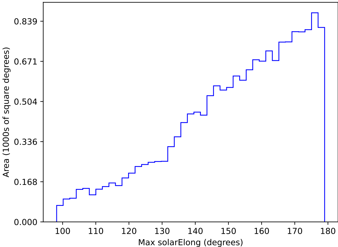
too_elab_r256_d3_ugrizy_v3.4_10yrs WFD g band: Max solarElong
