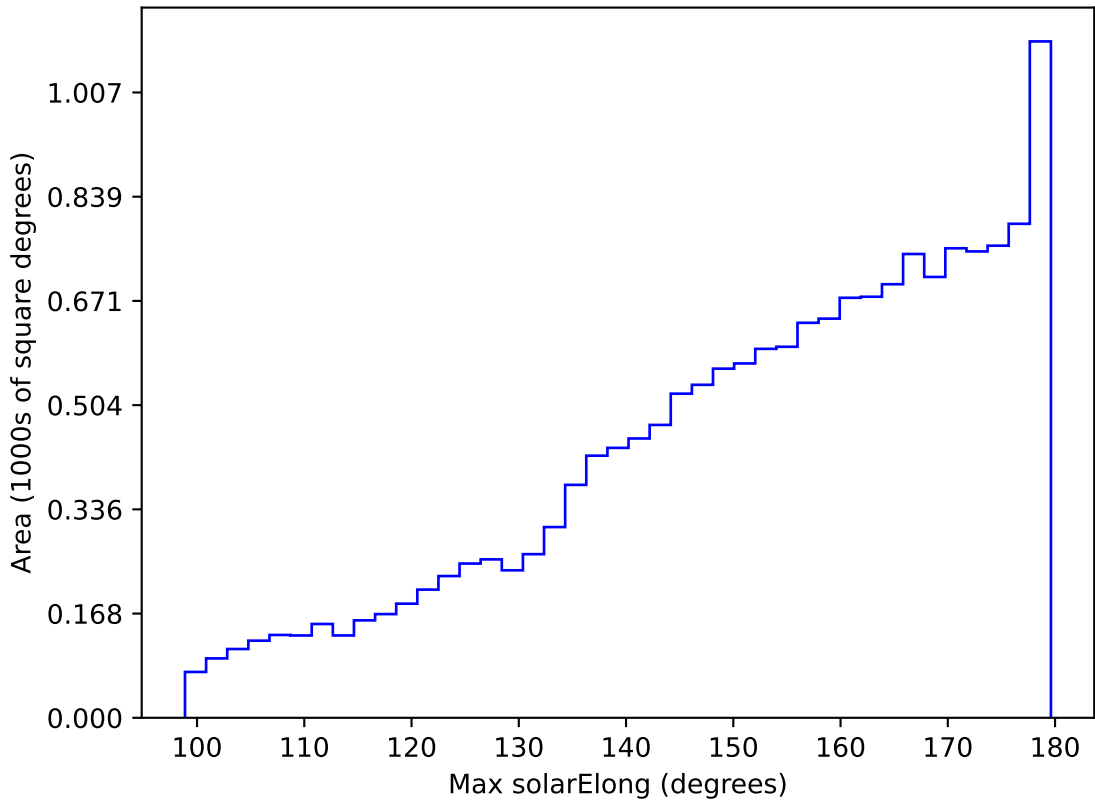
too_elab_r256_d3_ugrizy_v3.4_10yrs WFD all bands: Max solarElong
