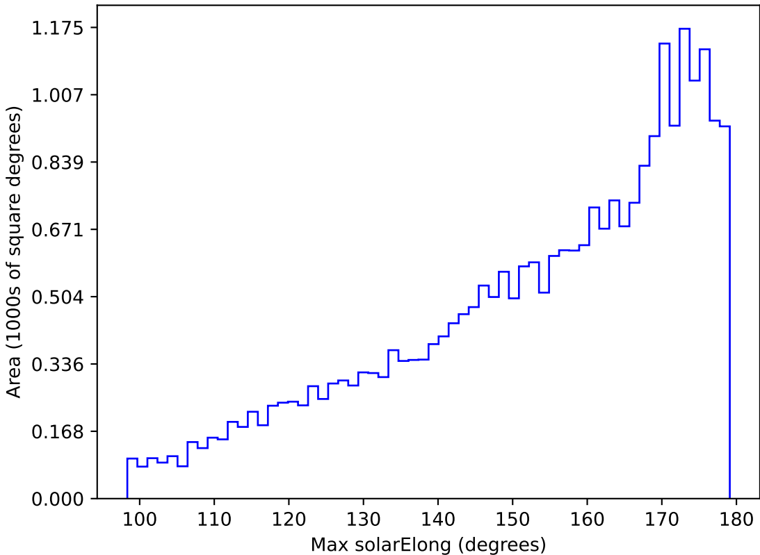
too_elab_r256_d3_ugrizy_v3.4_10yrs All sky g band: Max solarElong
