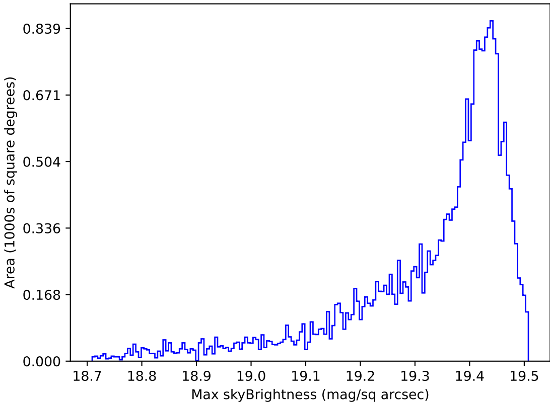
too_elab_r256_d3_ugrizy_v3.4_10yrs Yr 1 z band: Max skyBrightness
