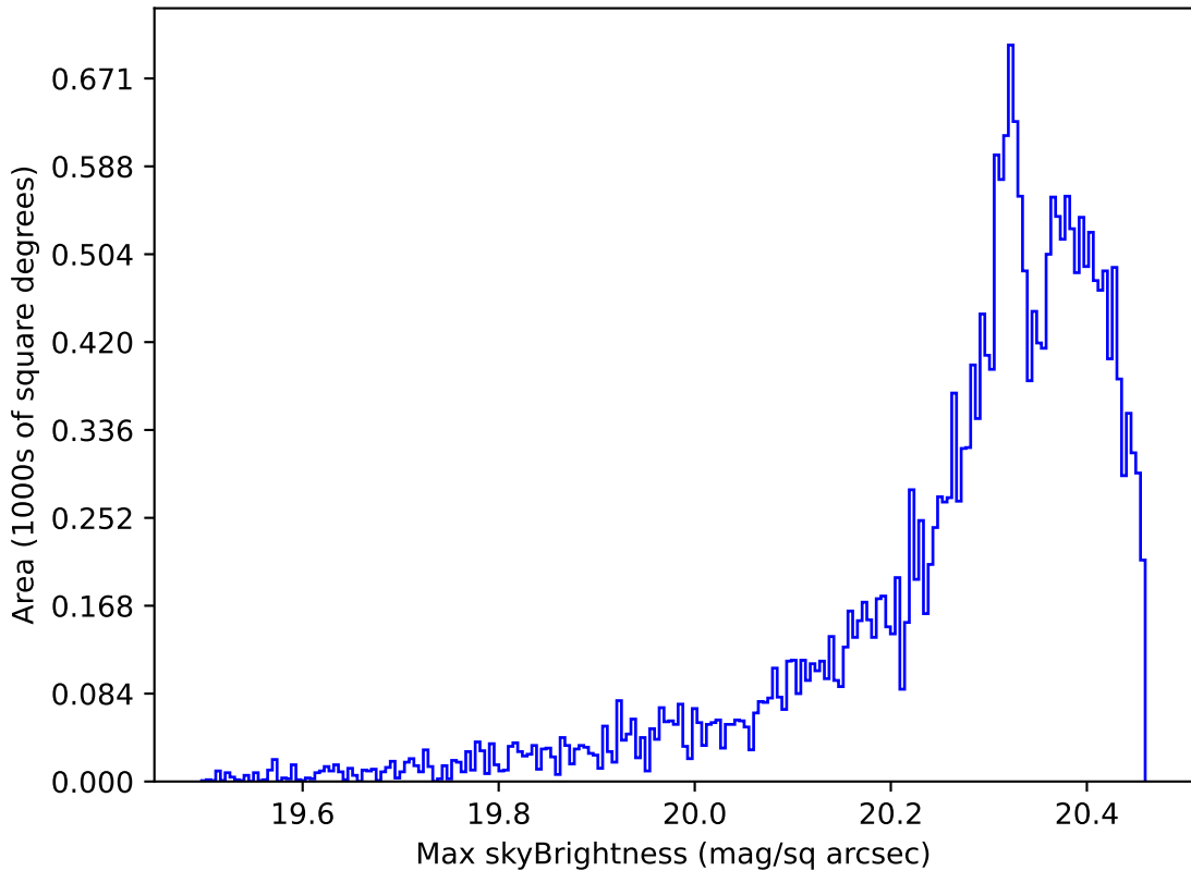
too_elab_r256_d3_ugrizy_v3.4_10yrs Yr 1 i band: Max skyBrightness
