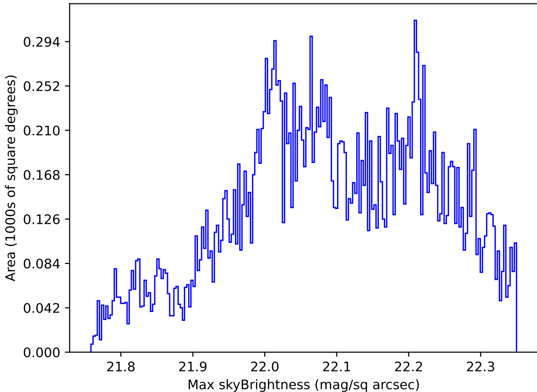
too_elab_r256_d3_ugrizy_v3.4_10yrs Yr 1 g band: Max skyBrightness
