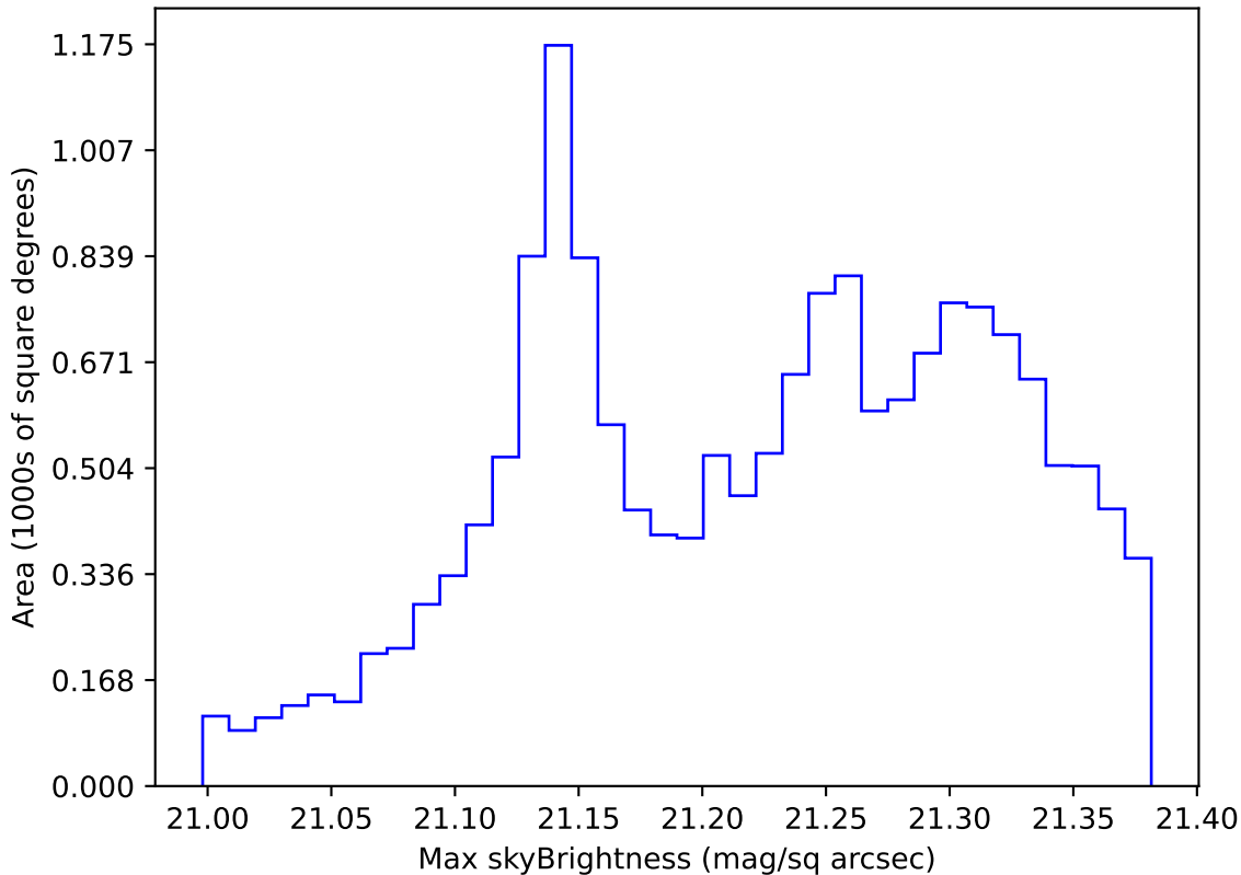
too_elab_r256_d3_ugrizy_v3.4_10yrs WFD r band: Max skyBrightness
