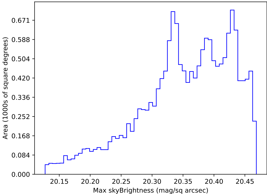
too_elab_r256_d3_ugrizy_v3.4_10yrs WFD i band: Max skyBrightness
