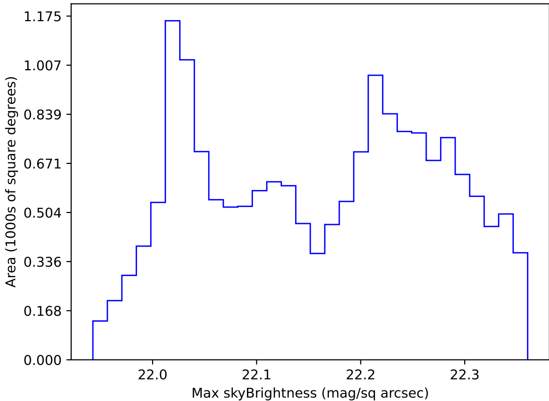
too_elab_r256_d3_ugrizy_v3.4_10yrs WFD g band: Max skyBrightness
