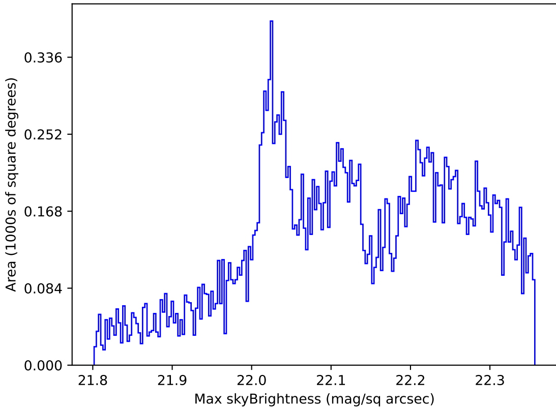
too_elab_r256_d3_ugrizy_v3.4_10yrs All sky g band: Max skyBrightness
