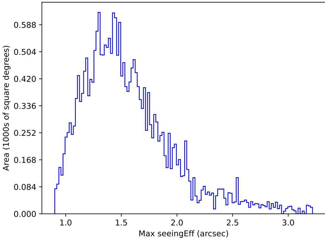
too_elab_r256_d3_ugrizy_v3.4_10yrs Yr 1 u band: Max seeingEff
