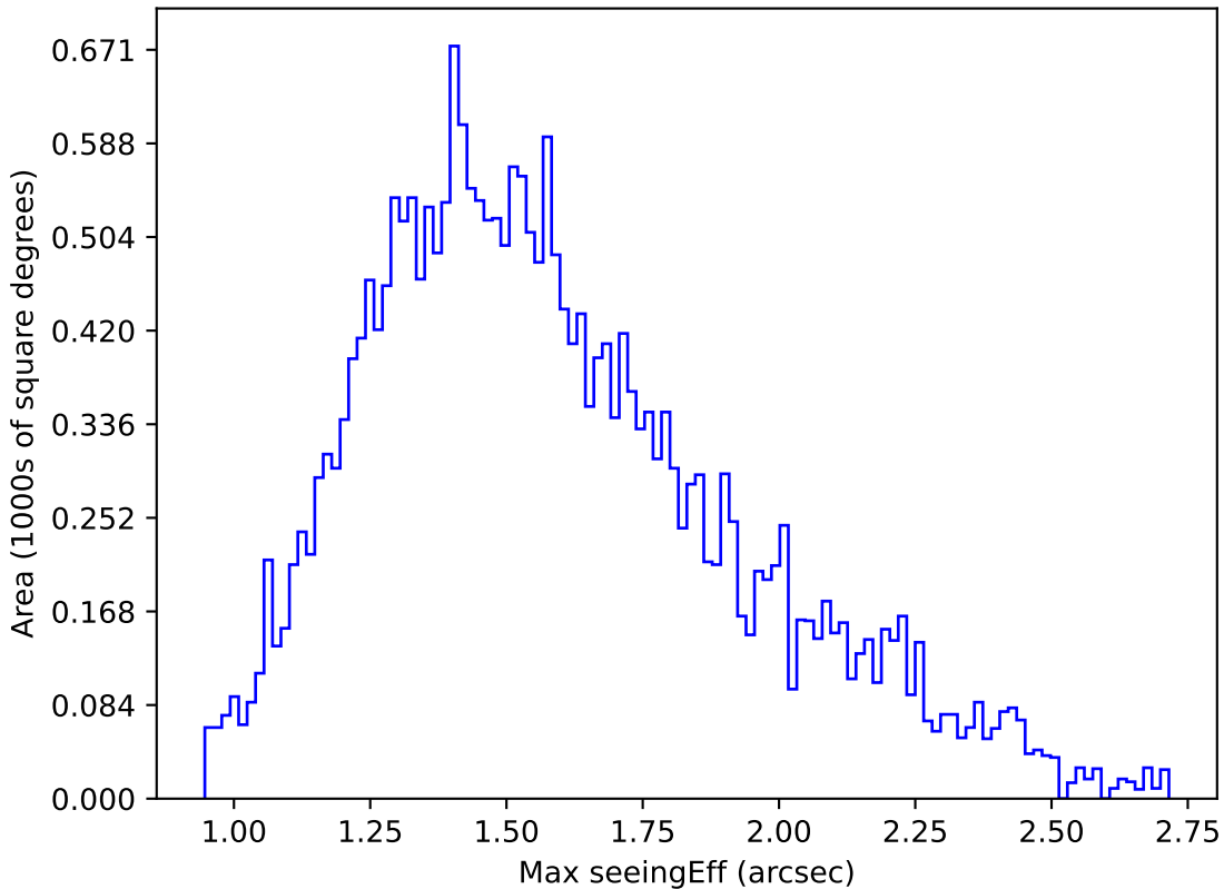
too_elab_r256_d3_ugrizy_v3.4_10yrs Yr 1 r band: Max seeingEff
