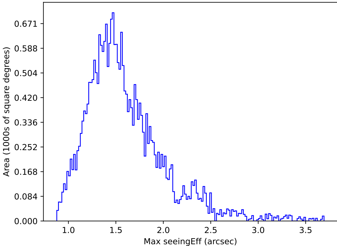
too_elab_r256_d3_ugrizy_v3.4_10yrs Yr 1 g band: Max seeingEff
