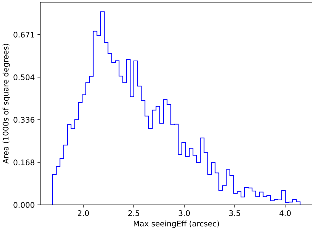
too_elab_r256_d3_ugrizy_v3.4_10yrs WFD u band: Max seeingEff
