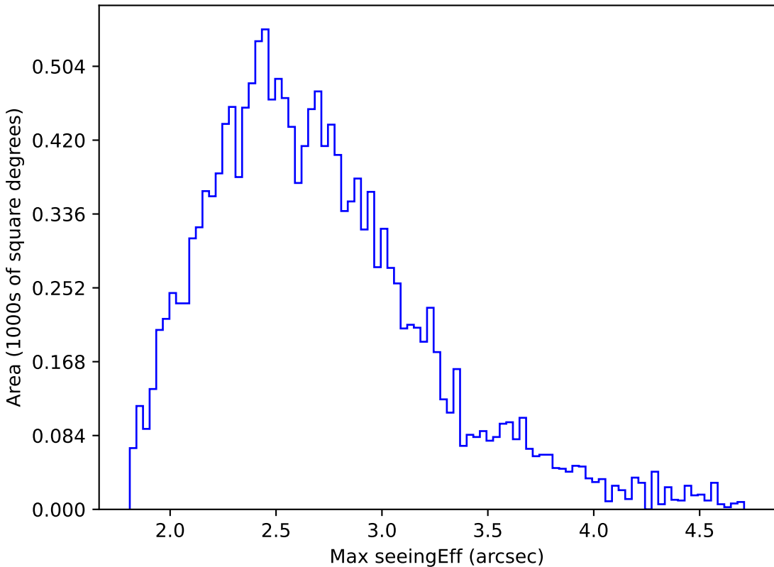
too_elab_r256_d3_ugrizy_v3.4_10yrs WFD r band: Max seeingEff
