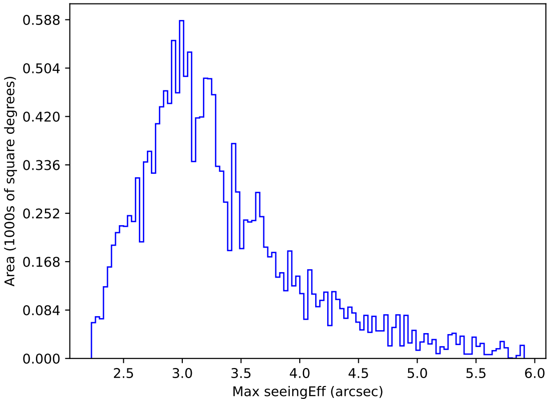
too_elab_r256_d3_ugrizy_v3.4_10yrs WFD all bands: Max seeingEff
