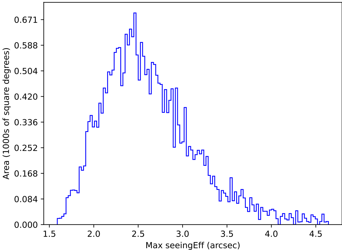
too_elab_r256_d3_ugrizy_v3.4_10yrs All sky r band: Max seeingEff
