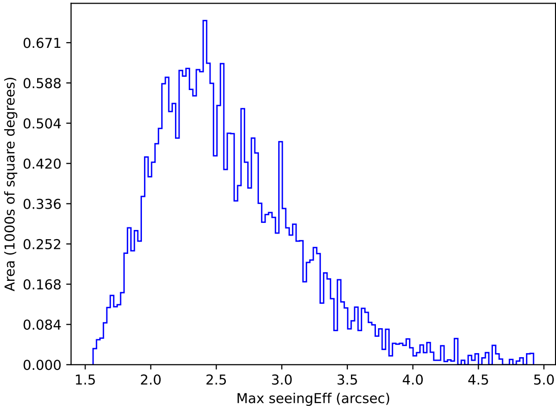
too_elab_r256_d3_ugrizy_v3.4_10yrs All sky i band: Max seeingEff
