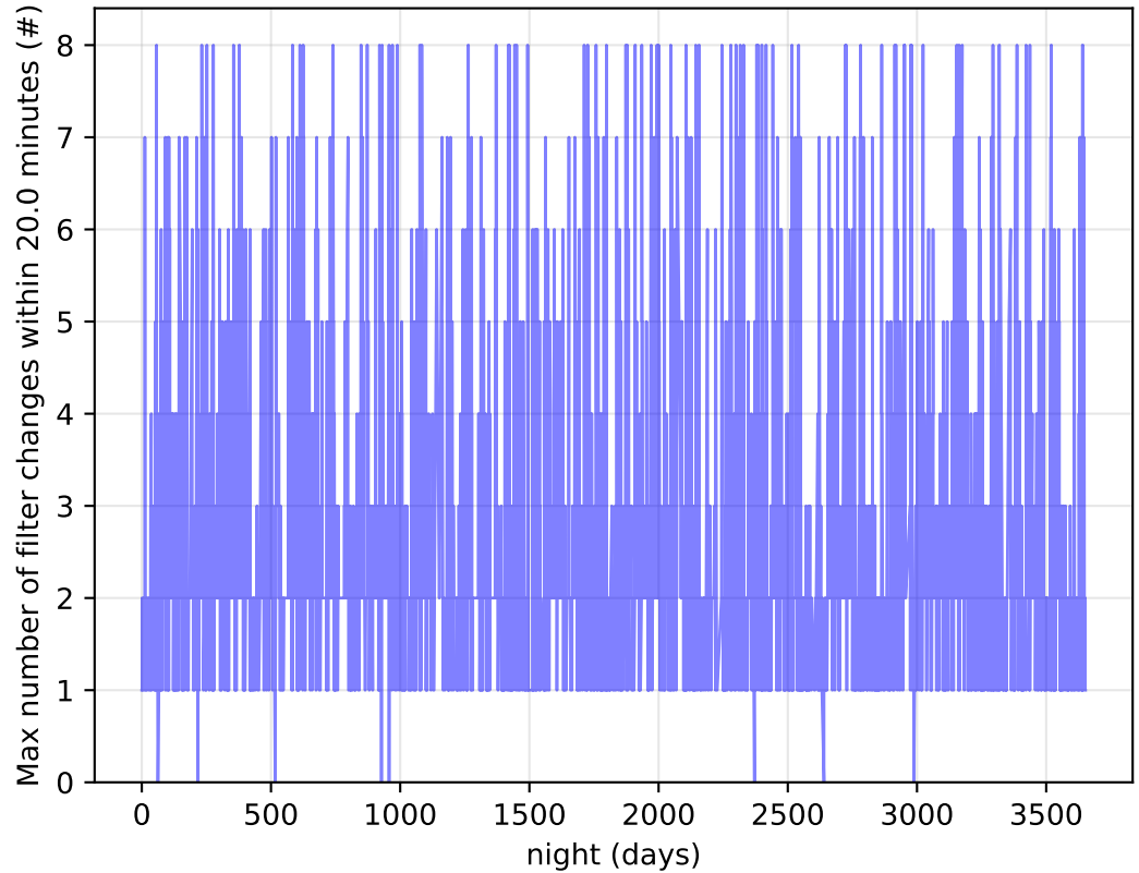
too_elab_r256_d3_ugrizy_v3.4_10yrs Per Night: Max number of filter changes within 20.0 minutes
