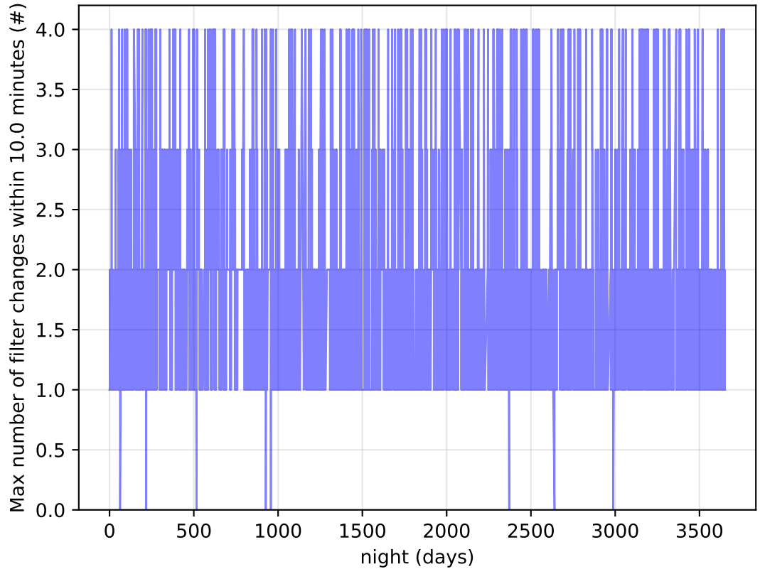
too_elab_r256_d3_ugrizy_v3.4_10yrs Per Night: Max number of filter changes within 10.0 minutes
