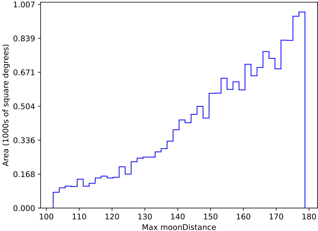
too_elab_r256_d3_ugrizy_v3.4_10yrs WFD u band: Max moonDistance
