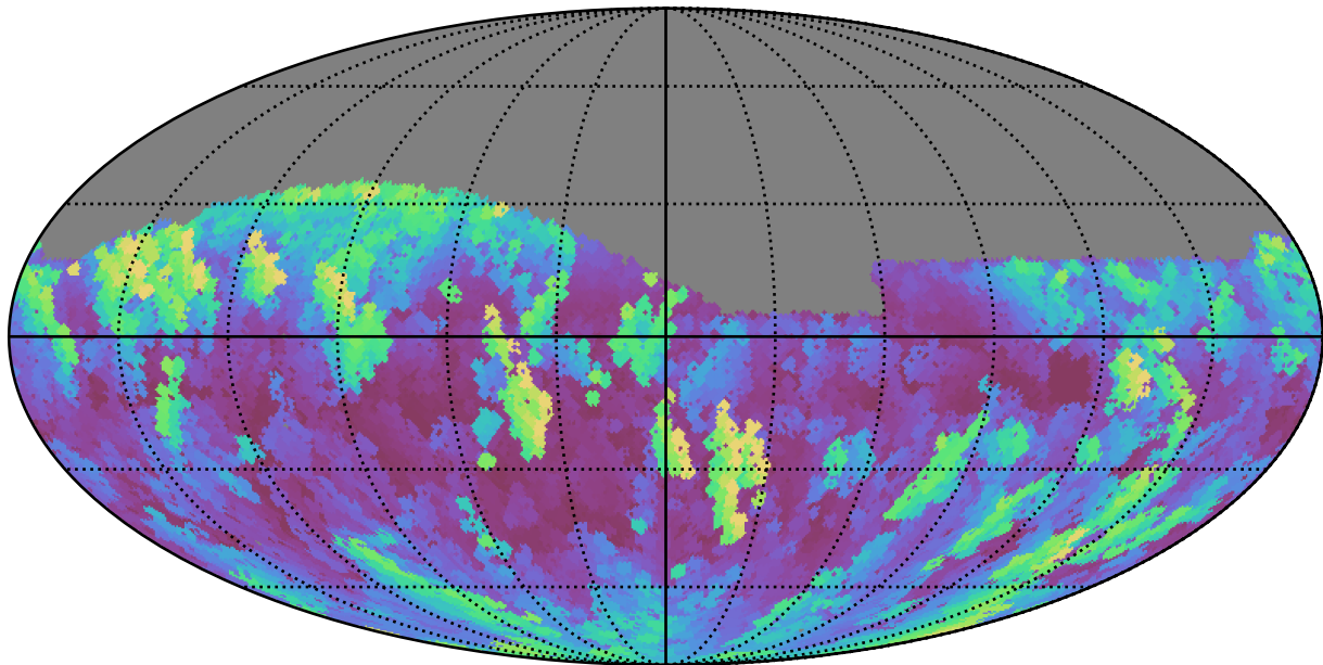
too_elab_r256_d3_ugrizy_v3.4_10yrs Yr 1 z band: Max airmass
