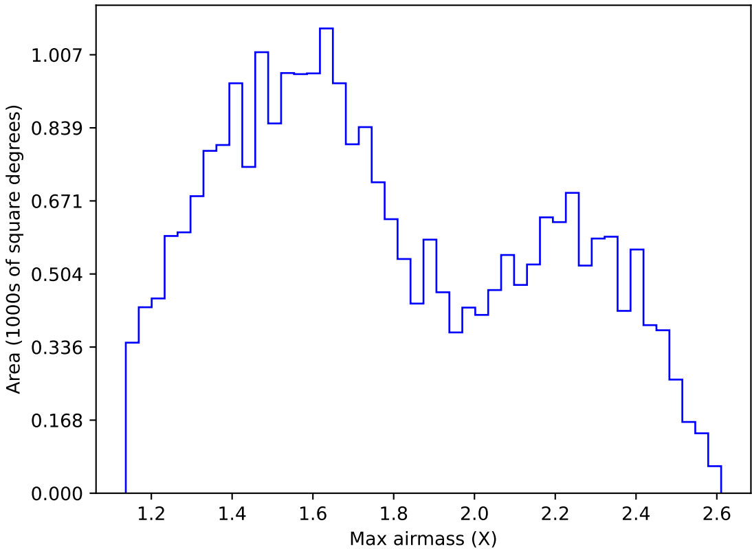
too_elab_r256_d3_ugrizy_v3.4_10yrs Yr 1 r band: Max airmass
