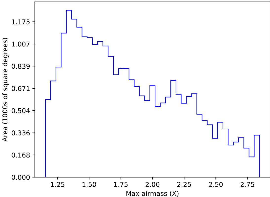
too_elab_r256_d3_ugrizy_v3.4_10yrs Yr 1 i band: Max airmass
