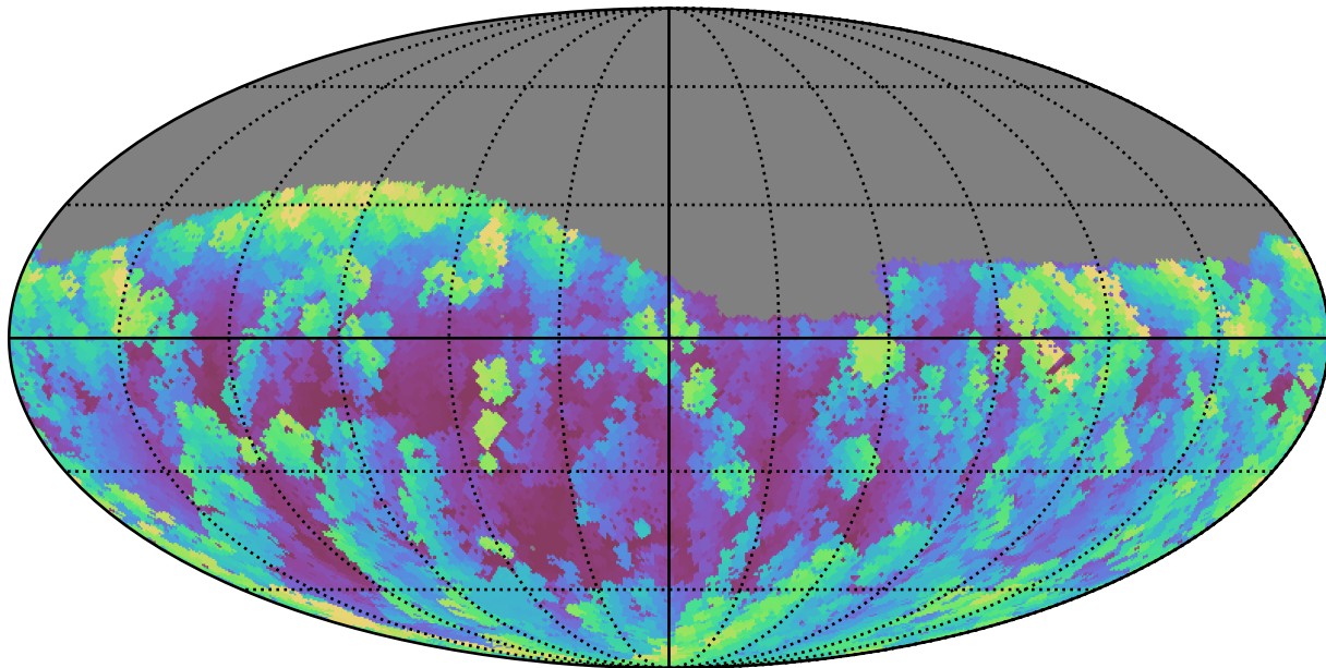
too_elab_r256_d3_ugrizy_v3.4_10yrs Yr 1 g band: Max airmass
