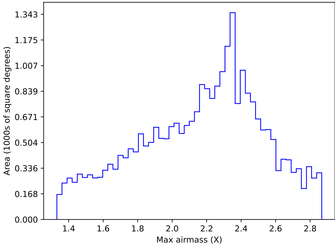
too_elab_r256_d3_ugrizy_v3.4_10yrs Yr 1 all bands: Max airmass
