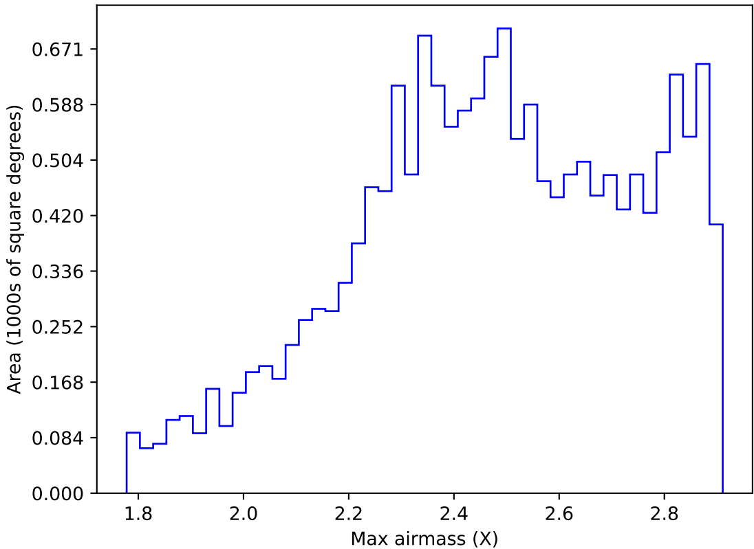
too_elab_r256_d3_ugrizy_v3.4_10yrs WFD z band: Max airmass
