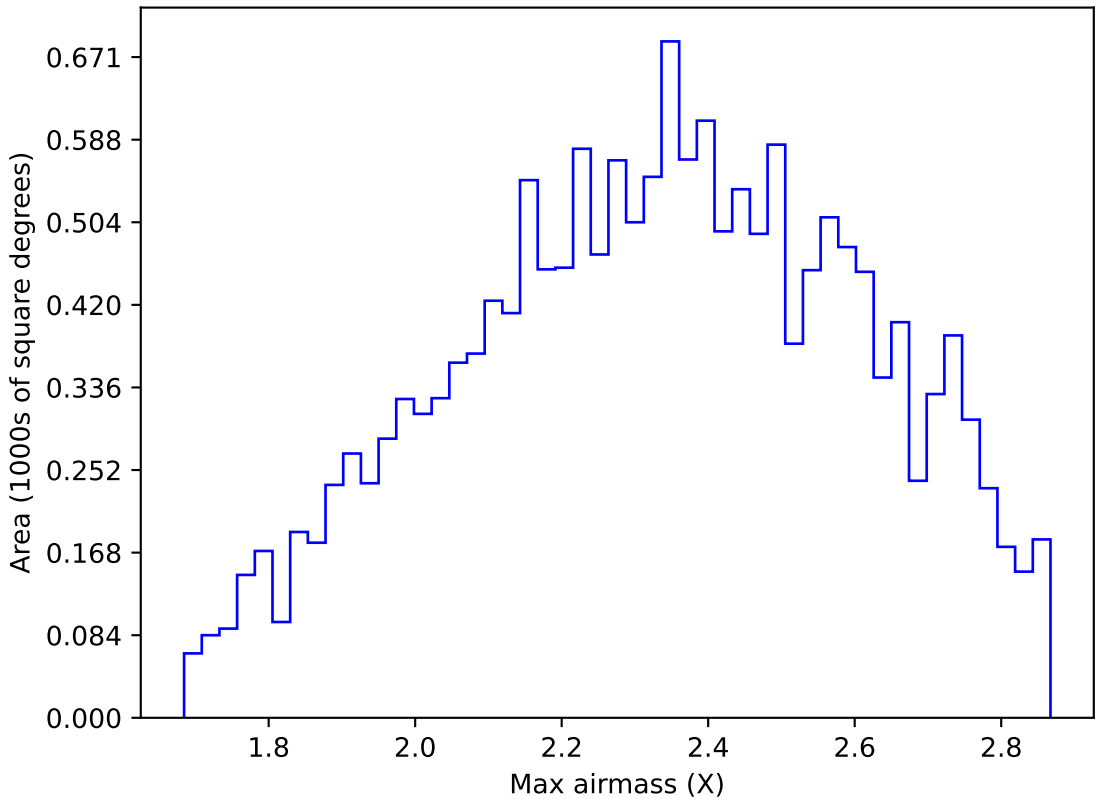
too_elab_r256_d3_ugrizy_v3.4_10yrs WFD y band: Max airmass
