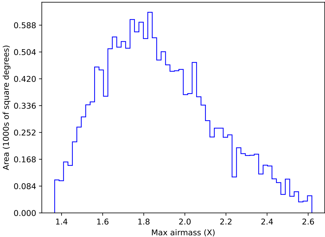
too_elab_r256_d3_ugrizy_v3.4_10yrs WFD u band: Max airmass
