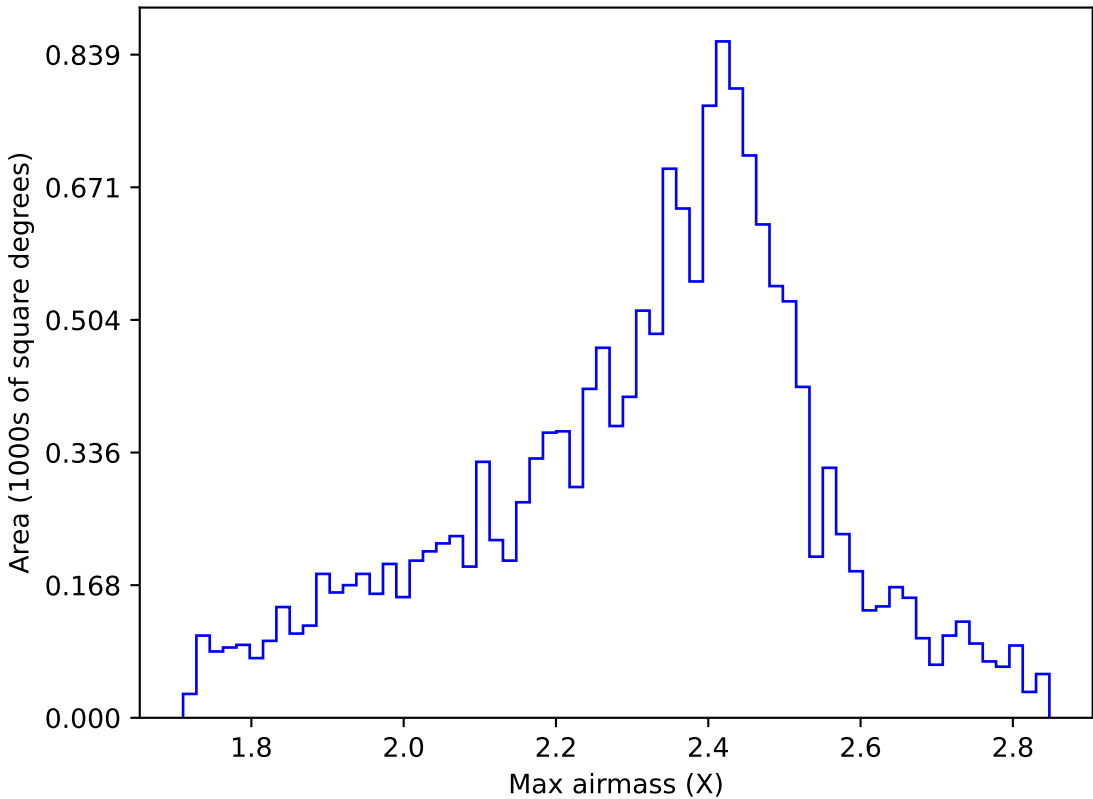
too_elab_r256_d3_ugrizy_v3.4_10yrs WFD r band: Max airmass
