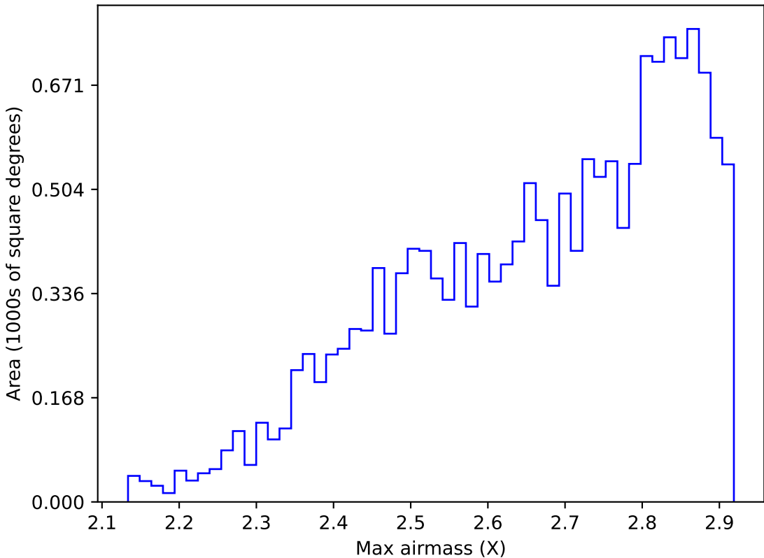
too_elab_r256_d3_ugrizy_v3.4_10yrs WFD all bands: Max airmass
