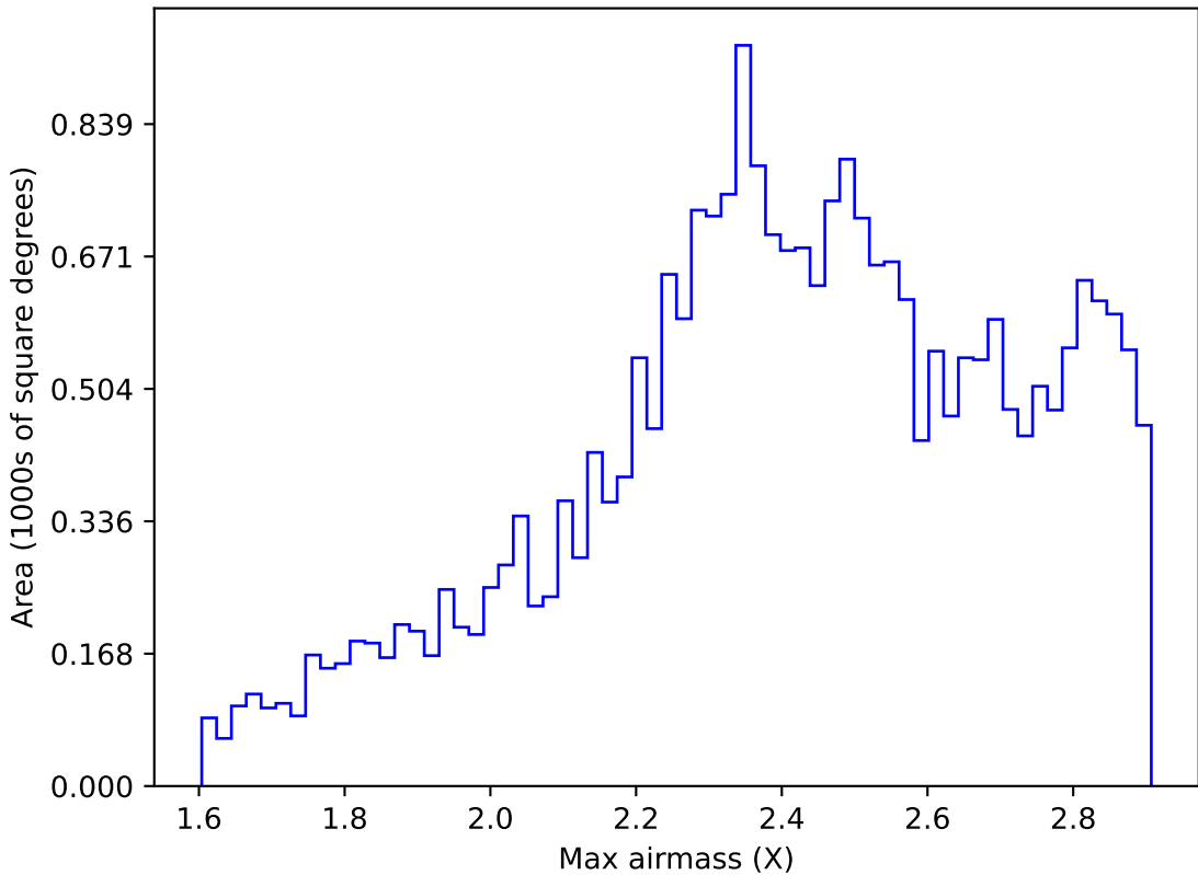
too_elab_r256_d3_ugrizy_v3.4_10yrs All sky z band: Max airmass
