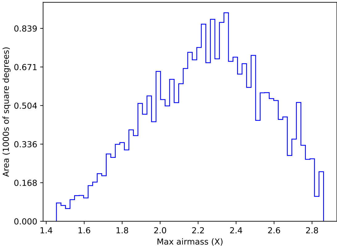
too_elab_r256_d3_ugrizy_v3.4_10yrs All sky y band: Max airmass
