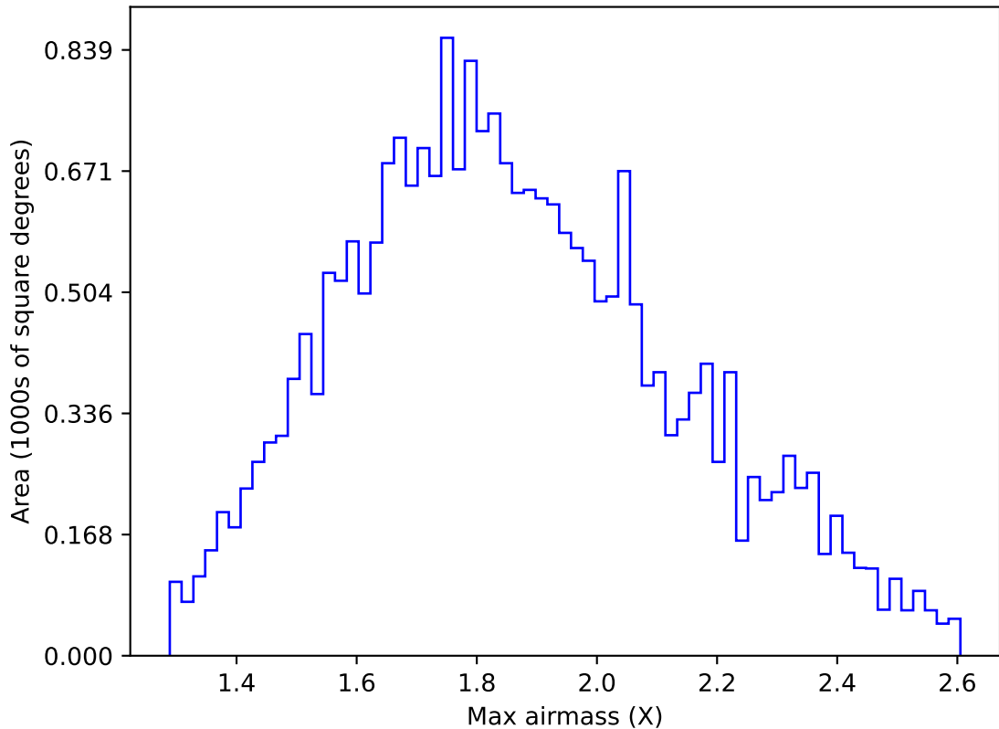
too_elab_r256_d3_ugrizy_v3.4_10yrs All sky u band: Max airmass
