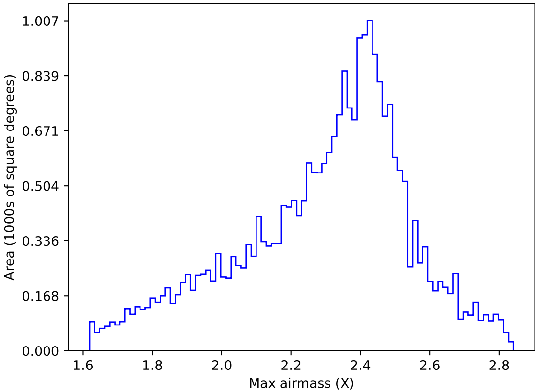
too_elab_r256_d3_ugrizy_v3.4_10yrs All sky r band: Max airmass
