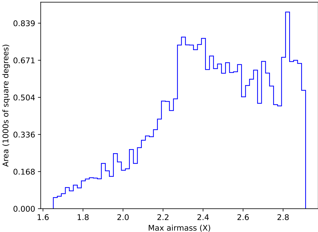
too_elab_r256_d3_ugrizy_v3.4_10yrs All sky i band: Max airmass
